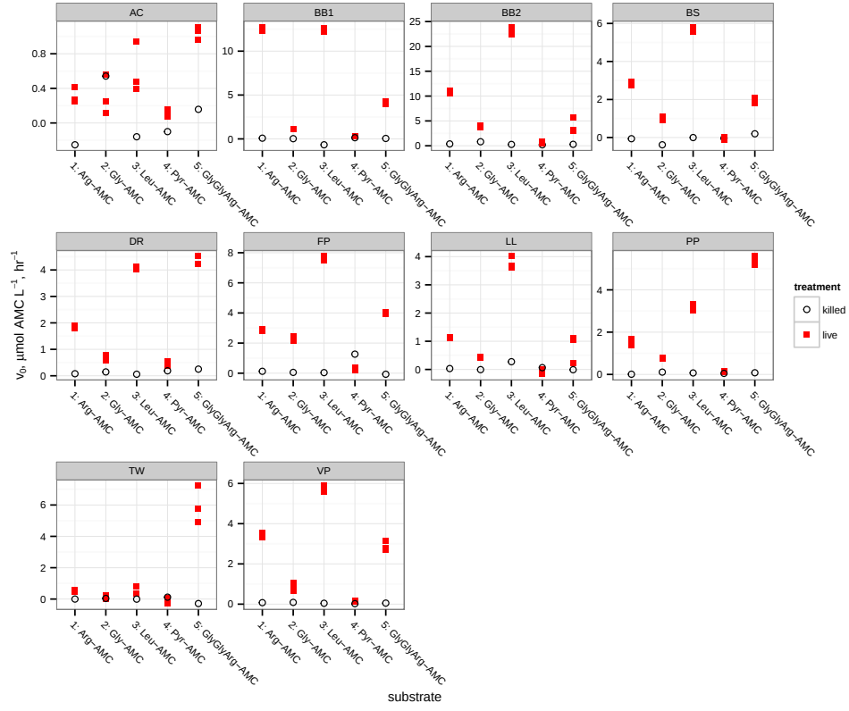
Figure 4: Activities of individual peptidases at each site.
