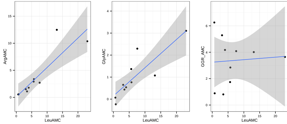
Figure 5: Hydrolysis rate of Leu-AMC vs Arg-AMC (left) and Leu-AMC vs GlyGlyArg-AMC
