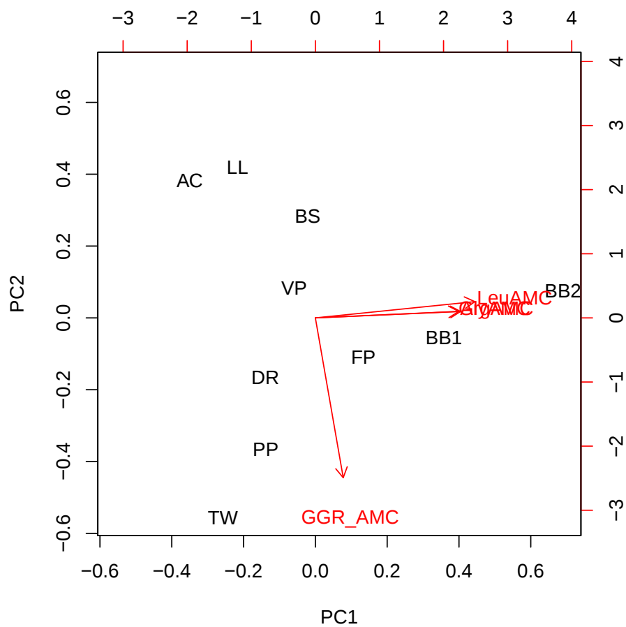
Figure 6: Principal components biplot of enzyme activities (Pyroglutamyl acid removed due because activities were generally below the detection limit).
