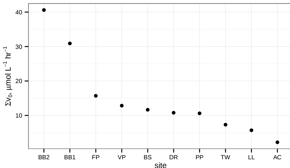
Figure 3: Summed activities of peptidases at each site.
